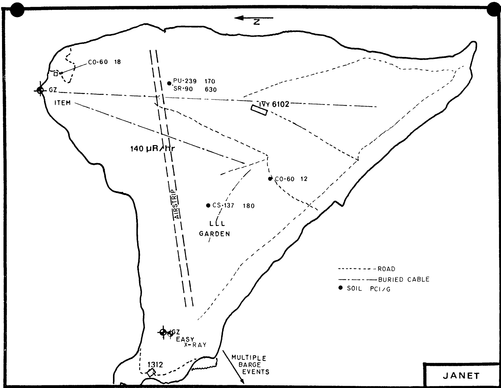
FIGURE 18. SITE JANET, PRINCIPAL FEATURES
